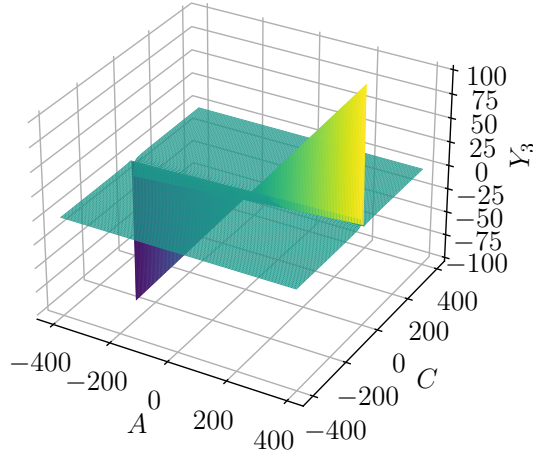
Figure 1: A vs C vs Y_3 , Example 3.1.
