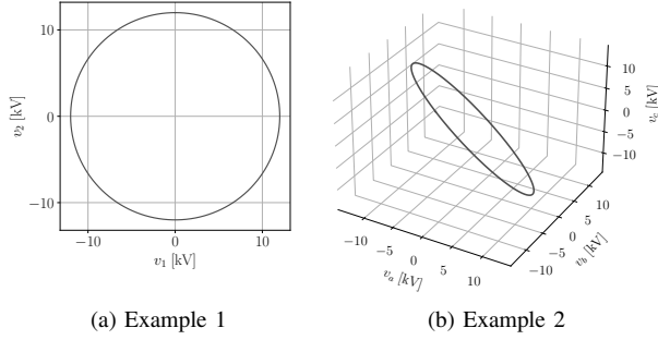
Fig. 1: Voltage ‘‘curves.’’
