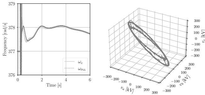
Fig. 3: Examples 7: Voltage and frequency at bus 26.
