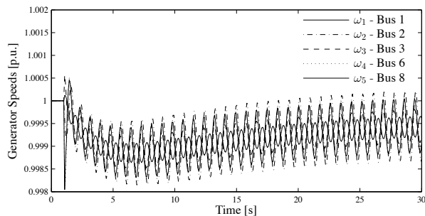
Fig. 12. Generator speed oscillations for the IEEE 14-bus test system due to Hopf bifurcation triggered by line outage at 40% overload.
