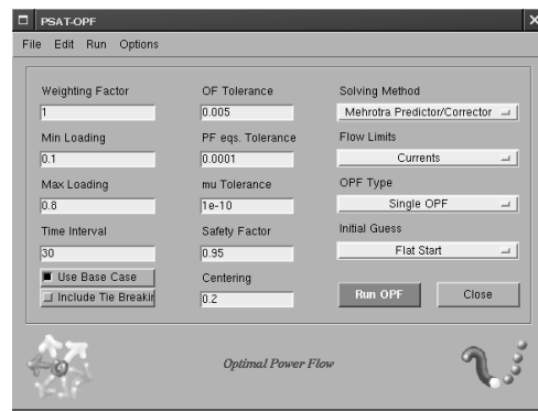
Fig. 11. GUI for OPF settings. Observe that the weighting factor is set to 1 in order to obtain the objective function (13).
