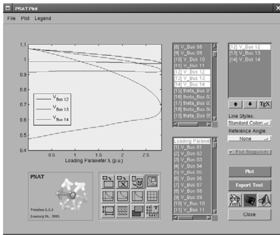
Fig. 9. GUI for plotting CPF results. The plots illustrate voltages at buses 12, 13 and 14 for the IEEE 14-bus test system with no contingency.
