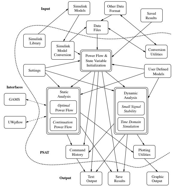
Fig. 1. Synoptic scheme of PSAT.
