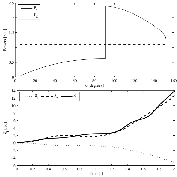
Fig. 4. Case A. OMIB plot and rotor angle trajectories for the WECC 3-machine, 9-bus system: first iteration of the TSC-OPF procedure. The system shows first-swing instability.
