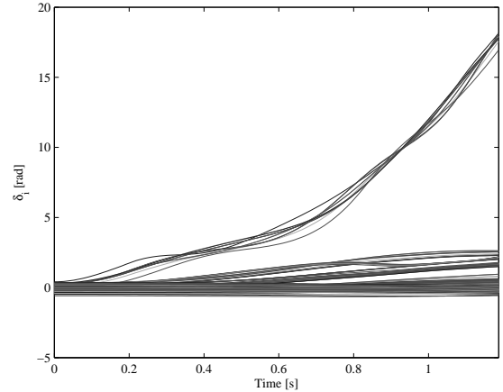
Fig. 10. Unstable trajectories of generator rotor angles for the 1228-bus system.
