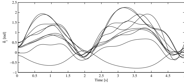
Fig. 9. Case D . Stable trajectories of generator rotor angles for the New England 39-bus system.
