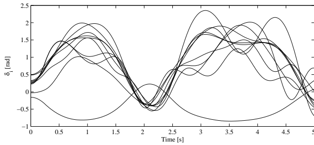
Fig. 8. Case C . Stable trajectories of generator rotor angles for the New England 39-bus system.
