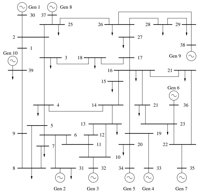
Fig. 7. One-line diagram of the New England 10-machine, 39-bus system.
