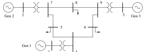
Fig. 2. One-line diagram of the WECC 3-machine, 9-bus system.
