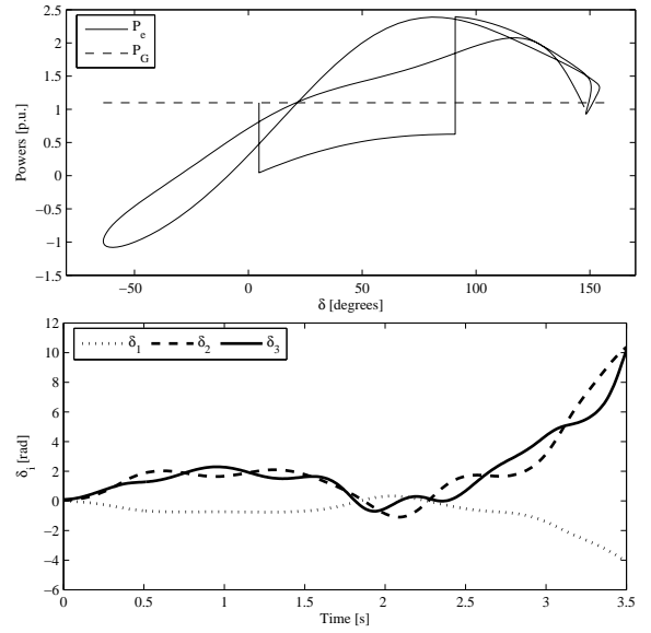
Fig. 5. Case A. OMIB plot and rotor angle trajectories for the WECC 3-machine, 9-bus system: second iteration of the TSC-OPF procedure. The system shows multi-swing instability.
