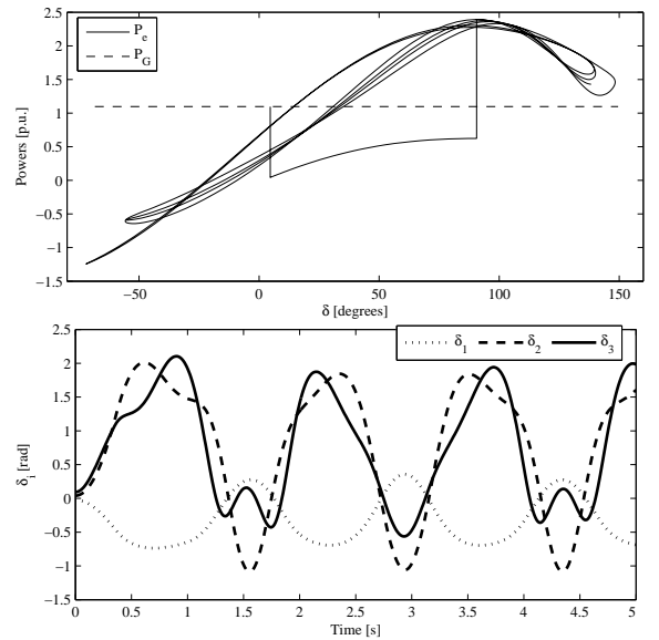
Fig. 6. Case A. OMIB plot and rotor angle trajectories for the WECC 3-machine, 9-bus system: third and final iteration of the TSC-OPF procedure. The system is stable.
