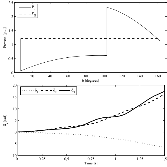
Fig. 3. Case A. OMIB plot and rotor angle trajectories for the WECC 3-machine, 9-bus system: unstable base case.
