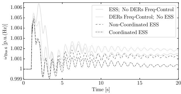
Fig. 8: Frequency response at bus 6 following the contingency.
