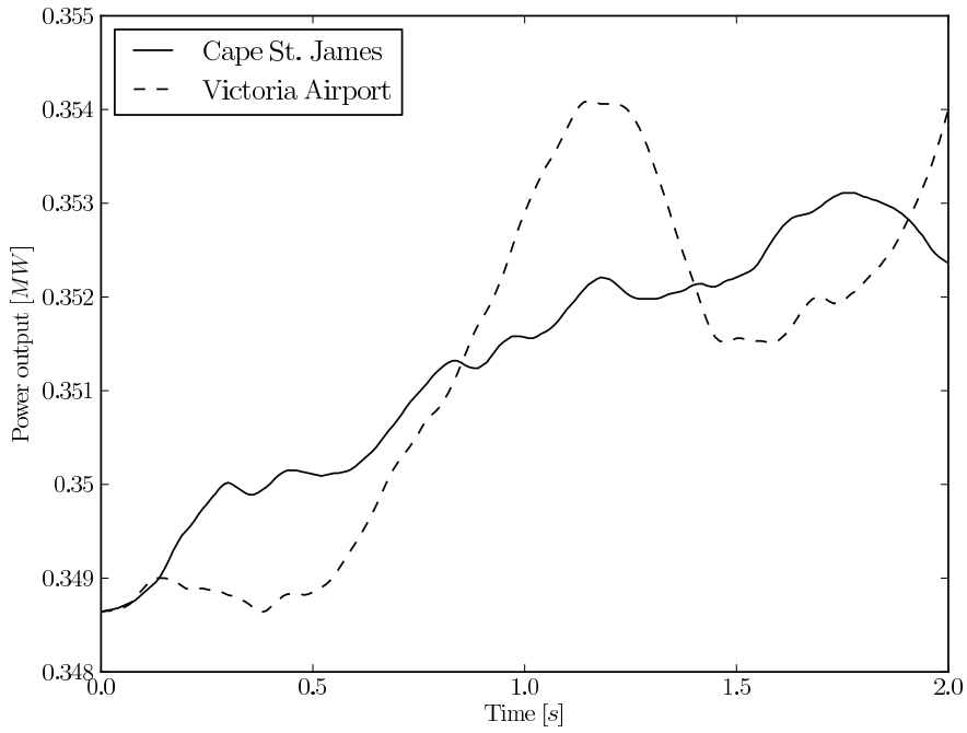
Fig. 7. Power output of a wind generator.
